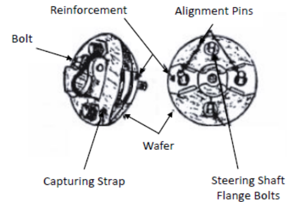
Figure 2 Typical Flexible Type Steering Coupling
