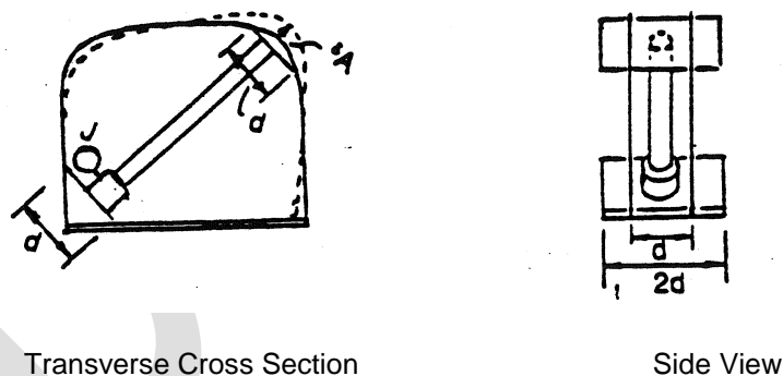
Figure 2. Arrangement of Hydraulic Jack for Rack-Loading of Two-Frame Assembly
